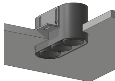
B) PROTRUDING INSTALLATION
